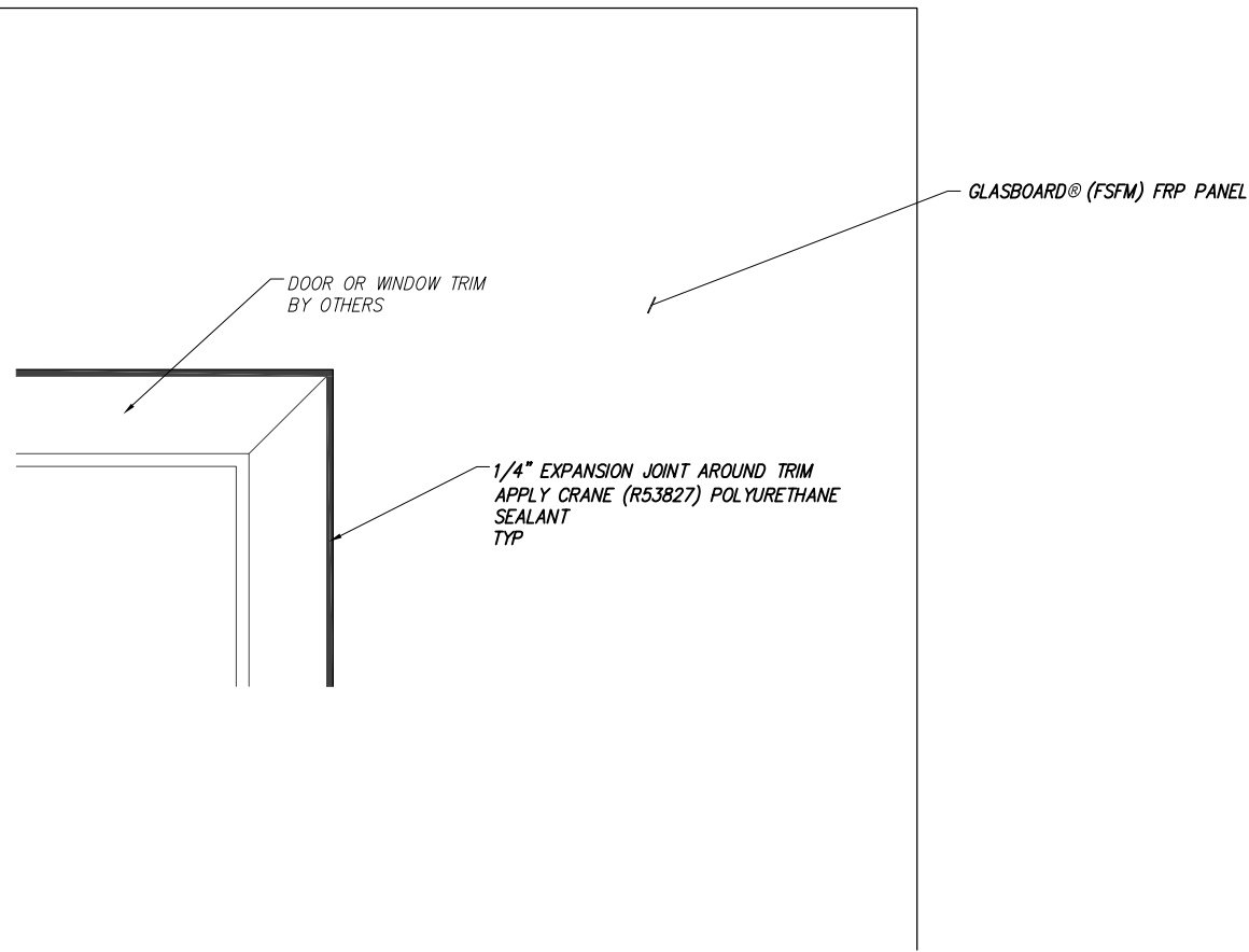
1 FRP PANEL AND DOOR TRIM SCALE: NOT TO SCALE
