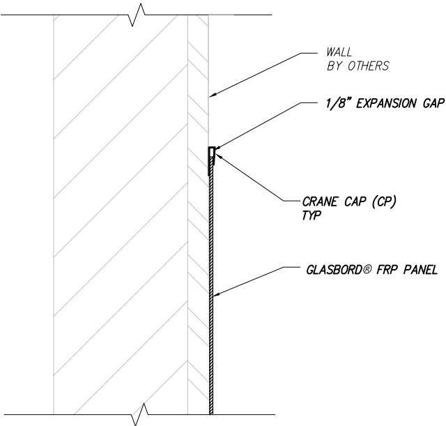
2 WAINSCOT JOINT DETAIL -- SCALE: NOT TO SCALE
