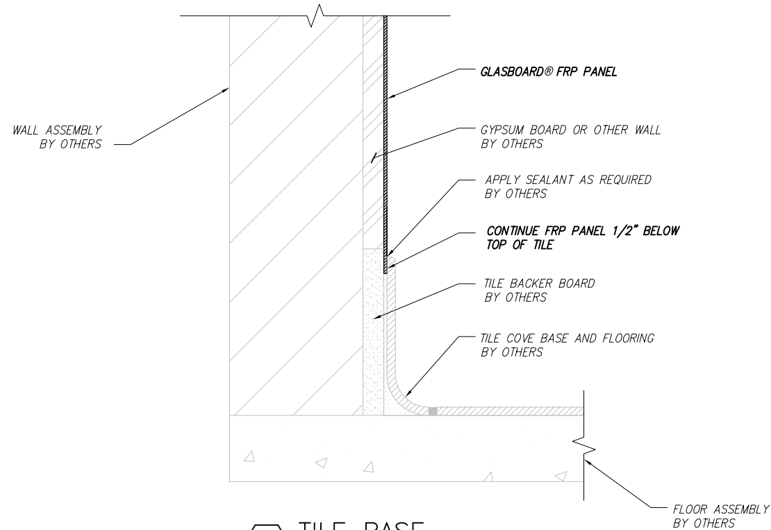
3 TILE BASE -- SCALE: NOT TO SCALE
