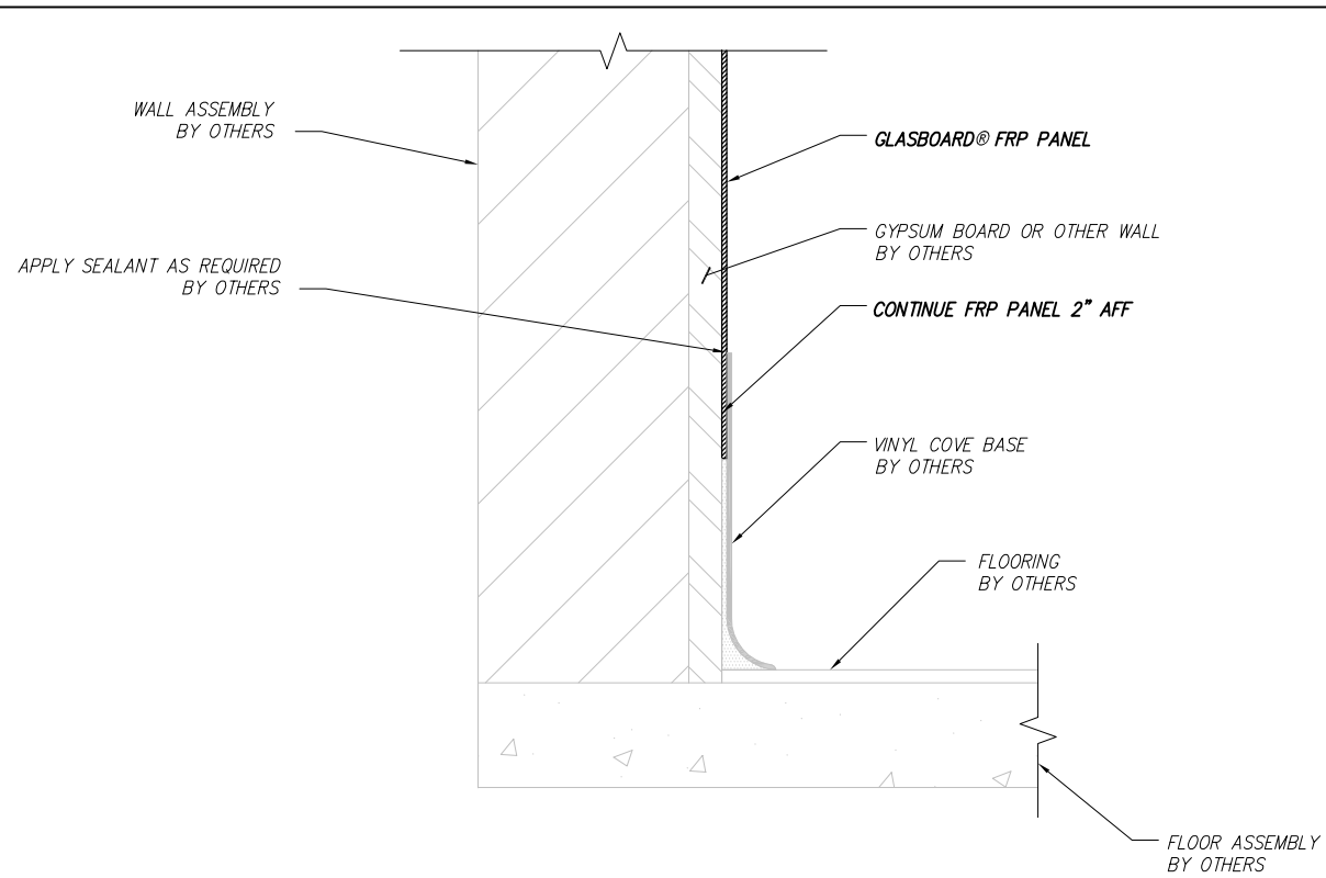
2 VINYL COVE BASE -- SCALE: NOT TO SCALE
